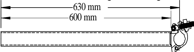
11 LF 02 Vertical hanger 600 long
