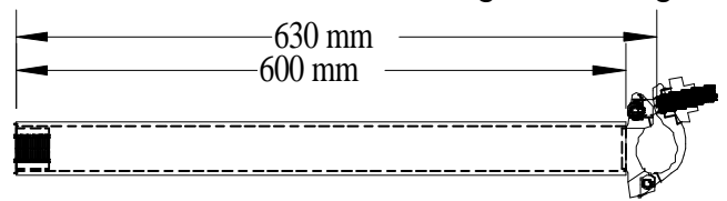
11 LF 04 Horizontal hanger 600 long
